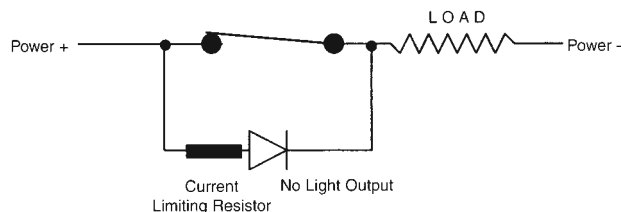
Figure 17. Wiring Diagram 2
