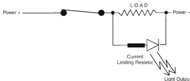
Figure 19. Wiring Diagram 4
