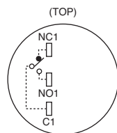
SPDT Contact (Single-pole/Double Throw)
