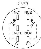
DPDT Contact (Double-pole/Double Throw)
