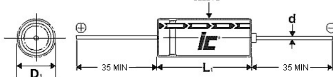
AXIAL LEAD 20V 50% RATED CAPACITOR ILLINOIS CAPACITOR COMPANY 2020 T2332
