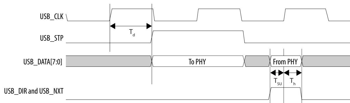
Figure 12. USB ULPI Timing Diagram
