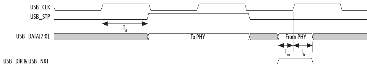
Figure 1-12: USB Timing Diagram
