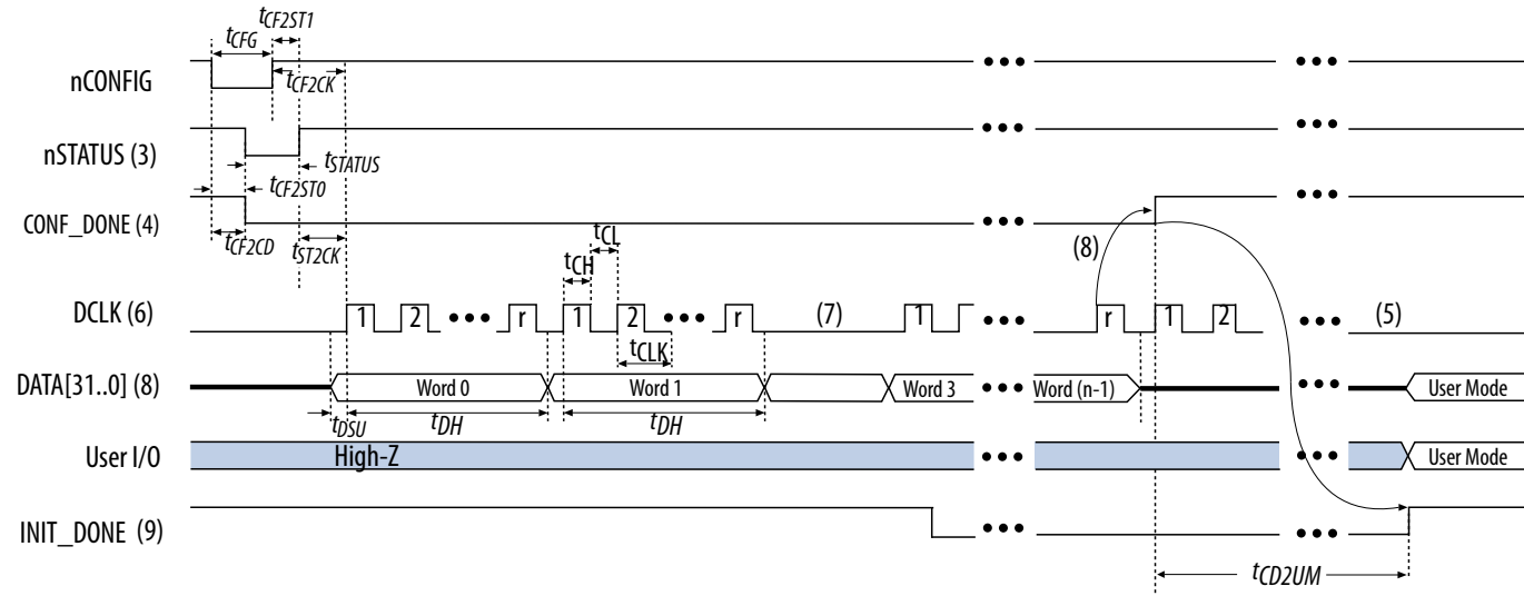
Figure 30. FPP Configuration Timing Waveform When the DCLK-to-DATA[] Ratio is &gt; 1 ,
