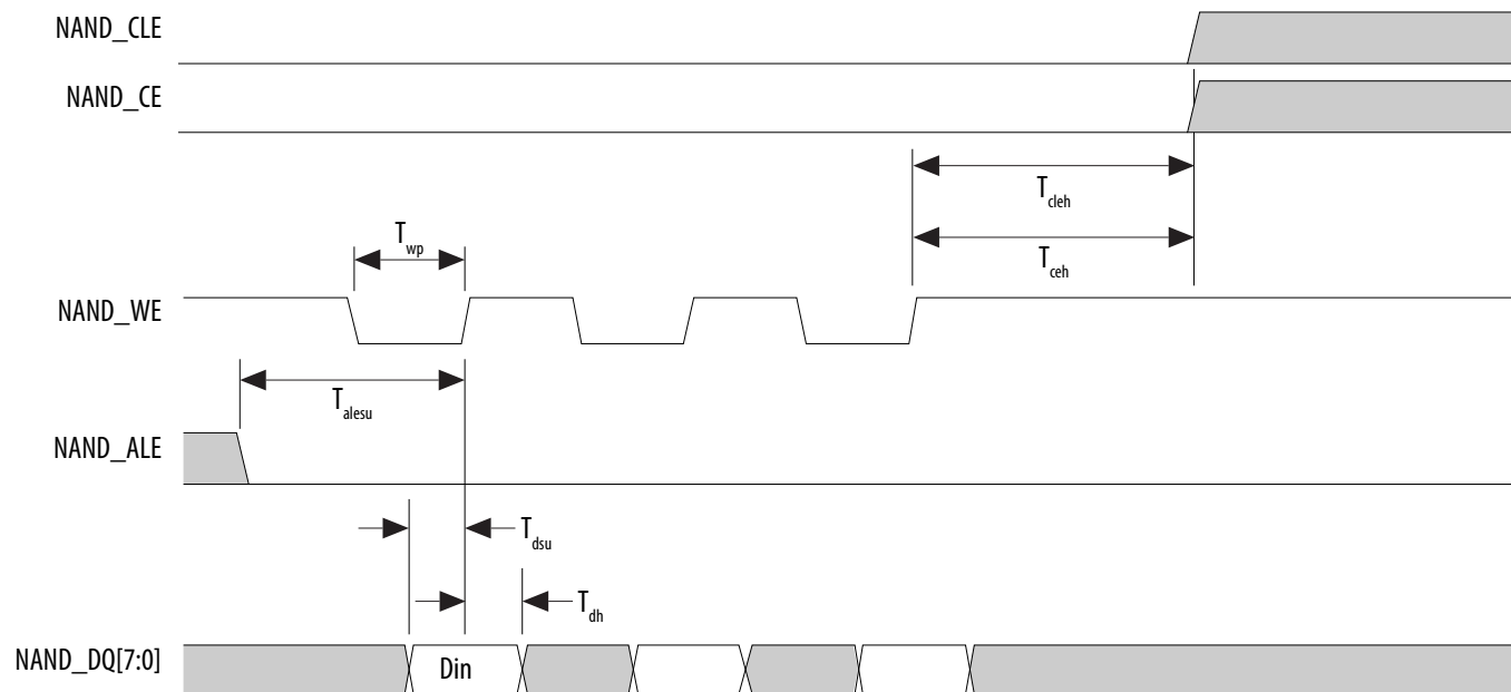
Figure 1-19: NAND Data Write Timing Diagram
