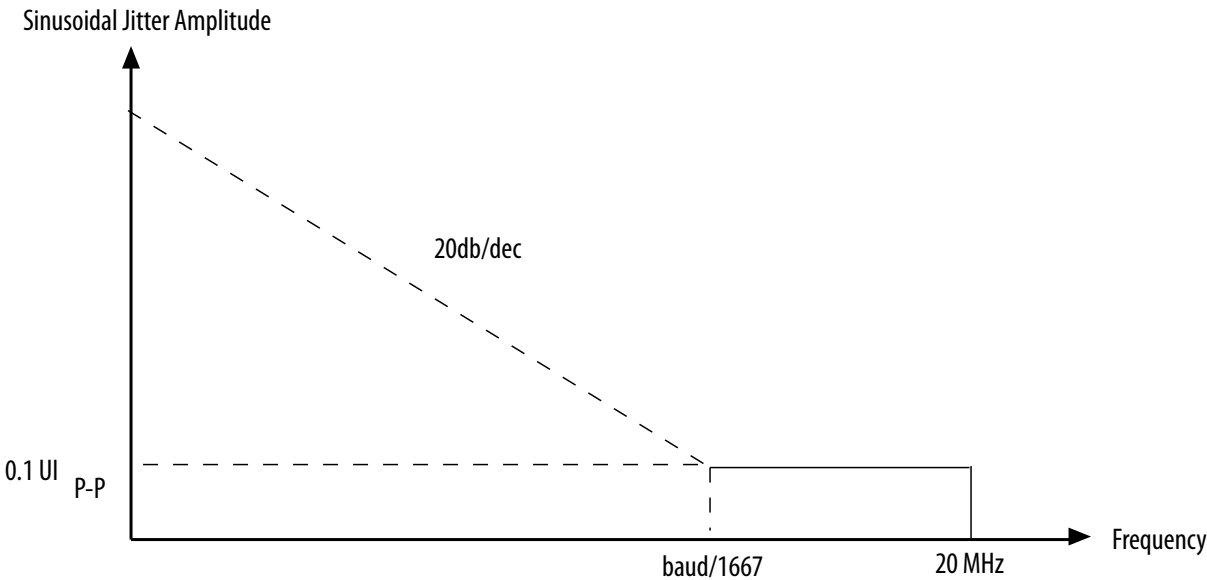
Figure 2-5: LVDS Soft-CDR/DPA Sinusoidal Jitter Tolerance Specification for a Data Rate < 1.25 Gbps
