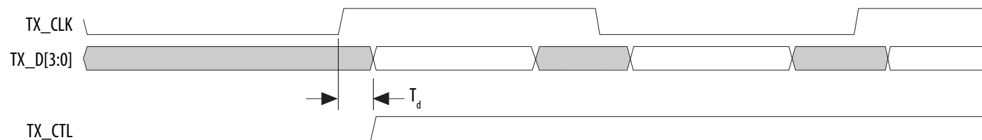
Figure 14. RGMI TX Timing Diagram
