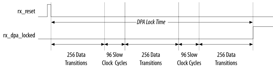
Figure 5. Dynamic Phase Alignment (DPA) Lock Time Specifications with DPA PLL Calibration Enabled
