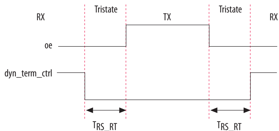
Figure 2-6: Timing Diagram for \text{oe} and \text{dyn\_term\_ctrl} Signals
