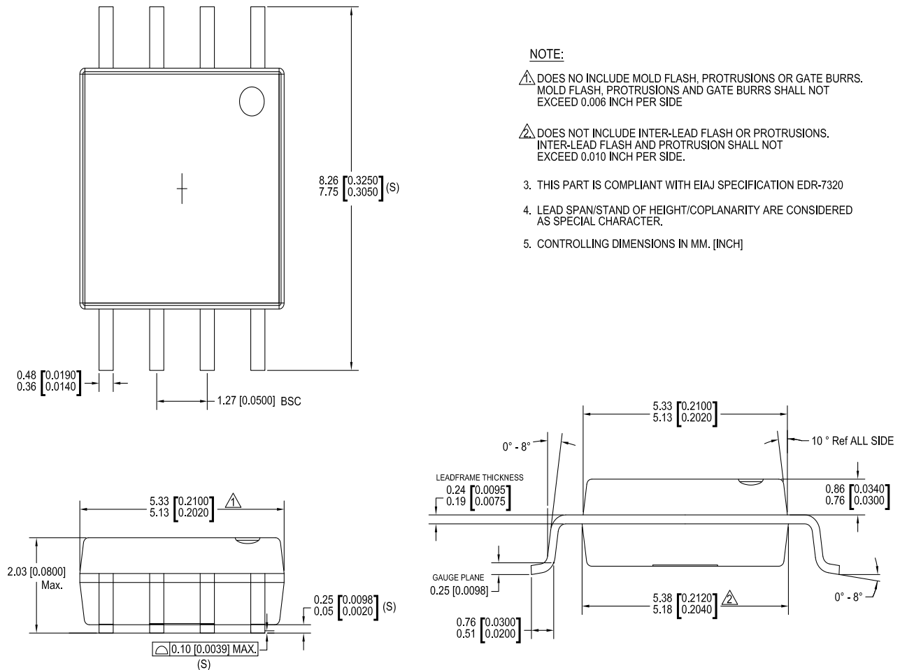
Figure 19. 8-Pin SOIC (208 Mils) Package Outline, 001-85261
