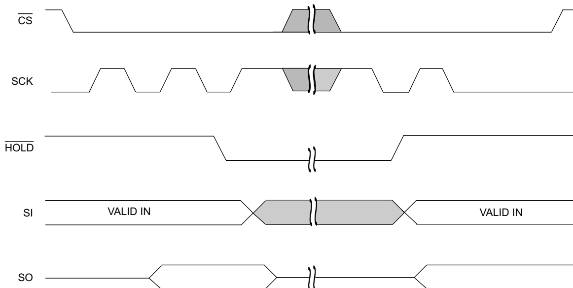
Figure 13. \overline{\text{HOLD}} Operation [2]
