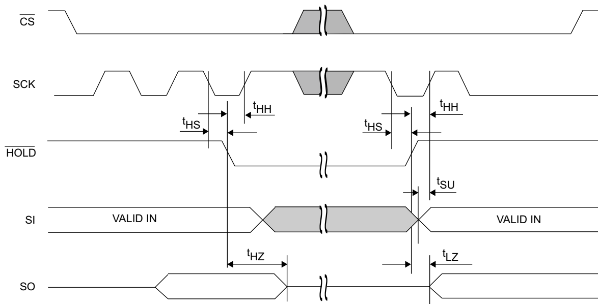
Figure 17. \overline{\text{HOLD}} Timing
