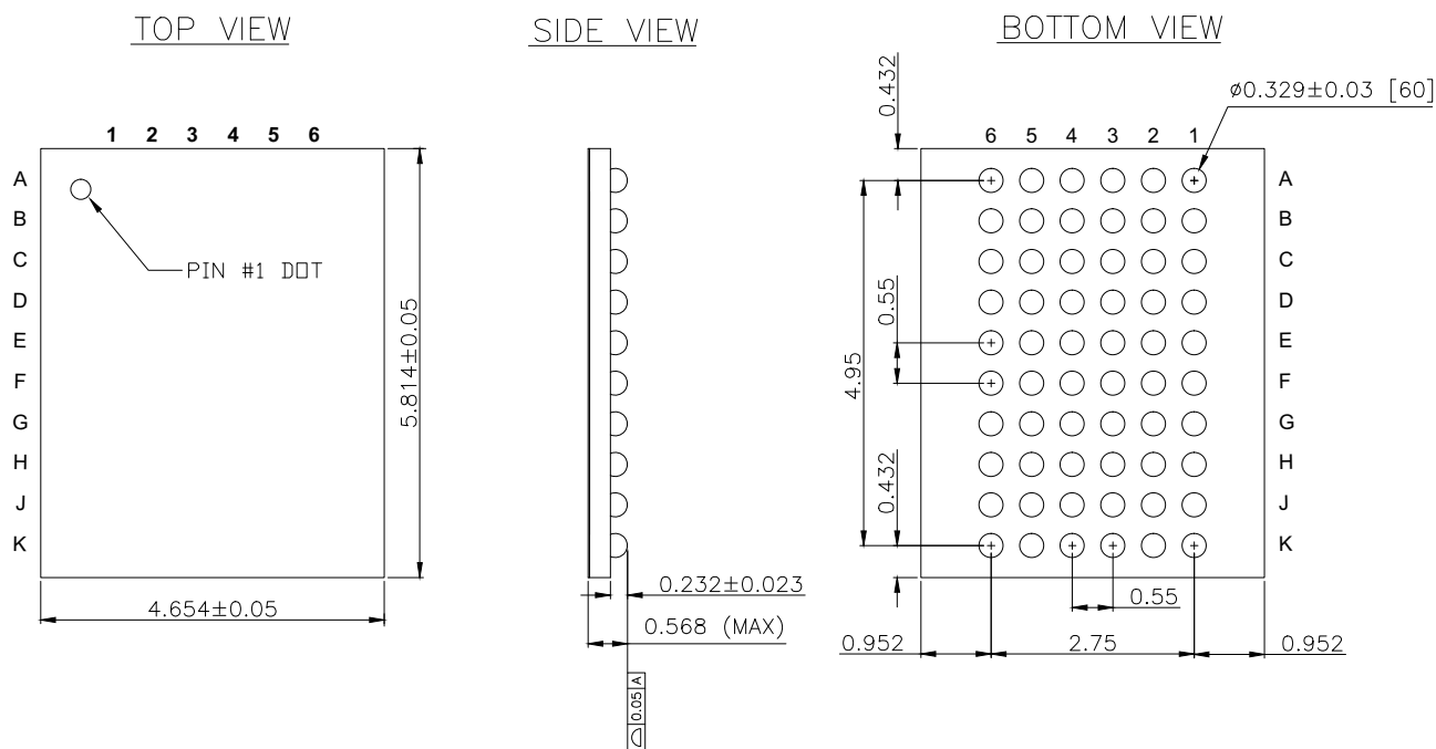
Figure 11. 60-Pin WLCSP Package Outline
