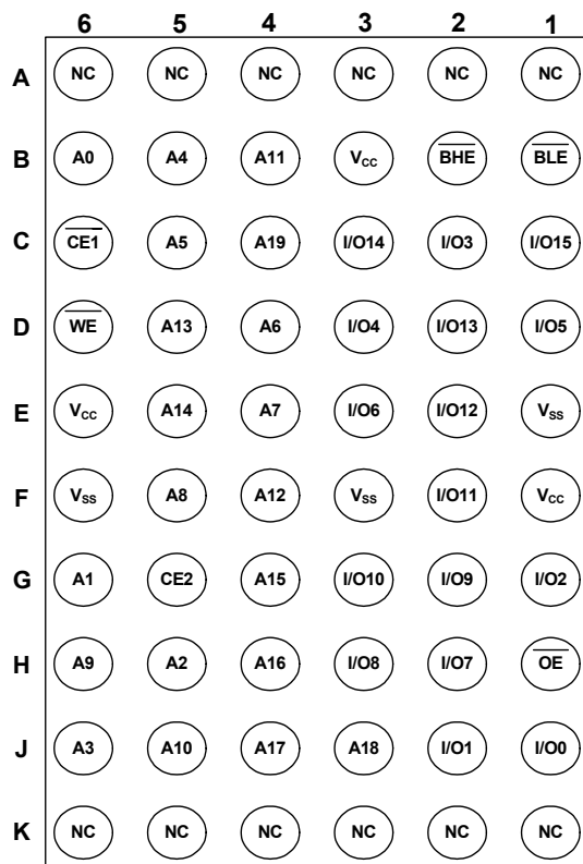
Figure 1. 60-Pin WLCSP Pinout (Ball Up View) [1]
