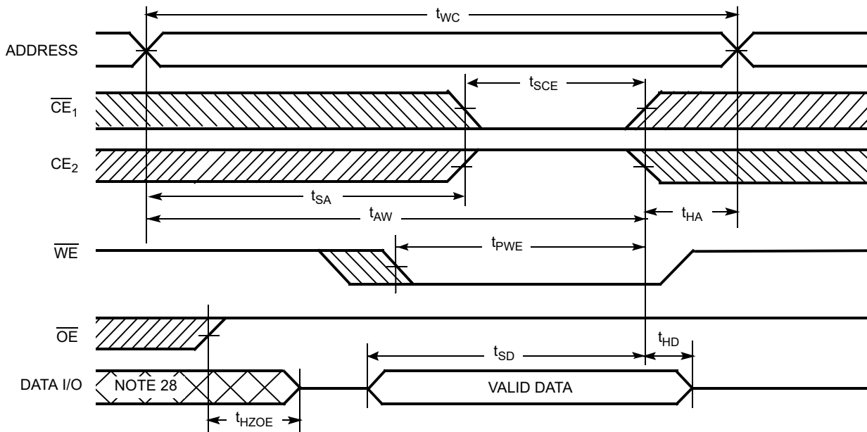
Figure 7. Write Cycle No. 2 ( \overline{\text{CE}}_1 or \text{CE}_2 Controlled) [25, 26, 27]
