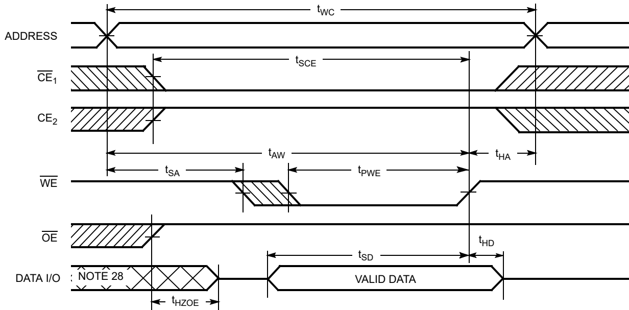
Figure 7. Write Cycle No. 2 ( \overline{\text{CE}}_1 or \text{CE}_2 Controlled) [25, 26, 27]
