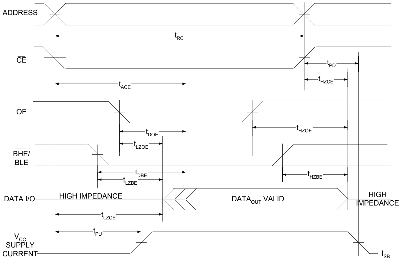
Figure 7. Read Cycle No. 2 ( \overline{\text{OE}} Controlled) [22, 23]
