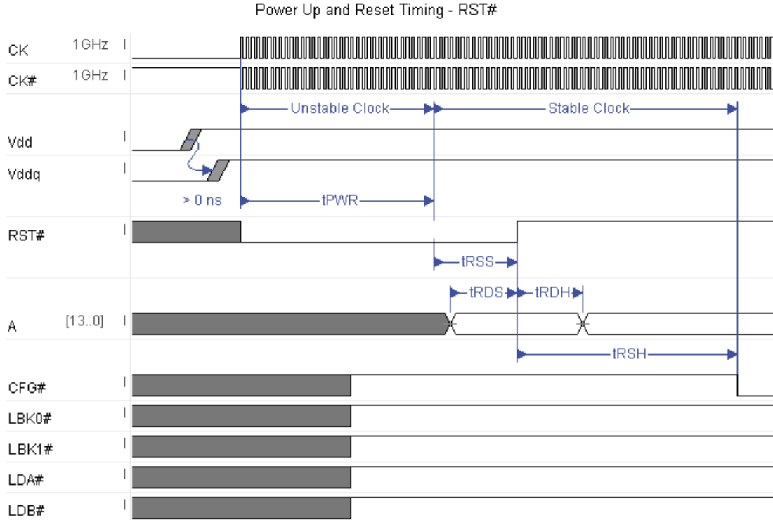
Figure 16. Reset Timings
