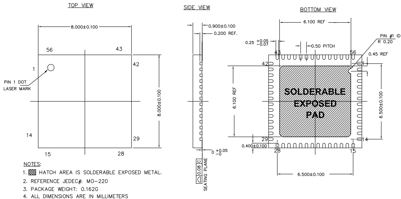
Figure 6. 56-pin QFN ( 8 \times 8 \times 1.0 mm) 6.1 \times 6.1 E-Pad (Sawn) Package Outline, 51-85187
