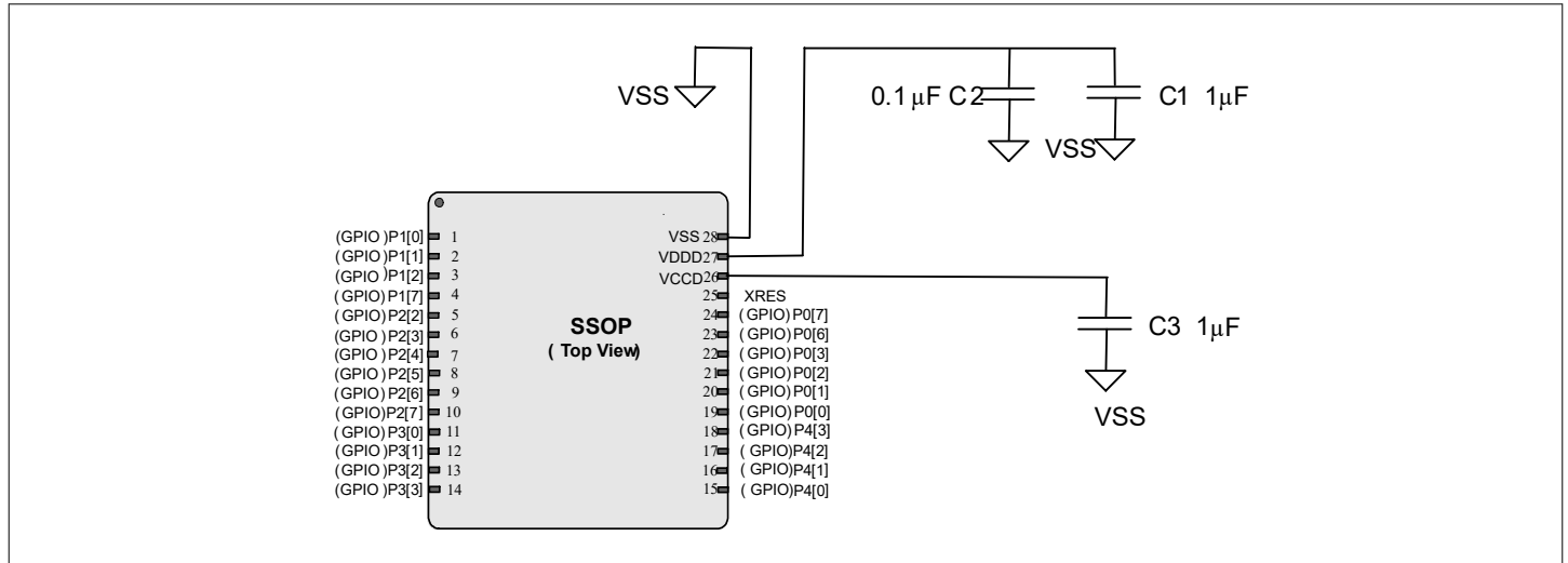
Figure 6 28-pin SSOP example
