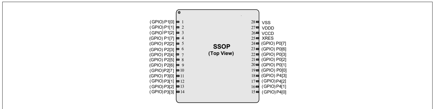
Figure 4 28-pin SSOP pinout
