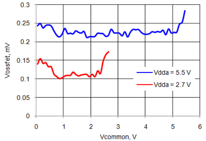
Figure 11-19. Opamp Voffset vs V_{common} and V_{DDA} , 25\text{ }^{\circ}\text{C}
