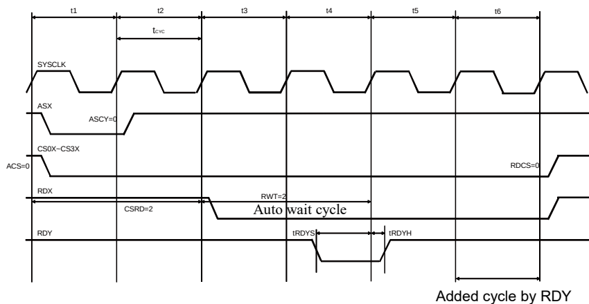
External bus I/F (ready) Timing
