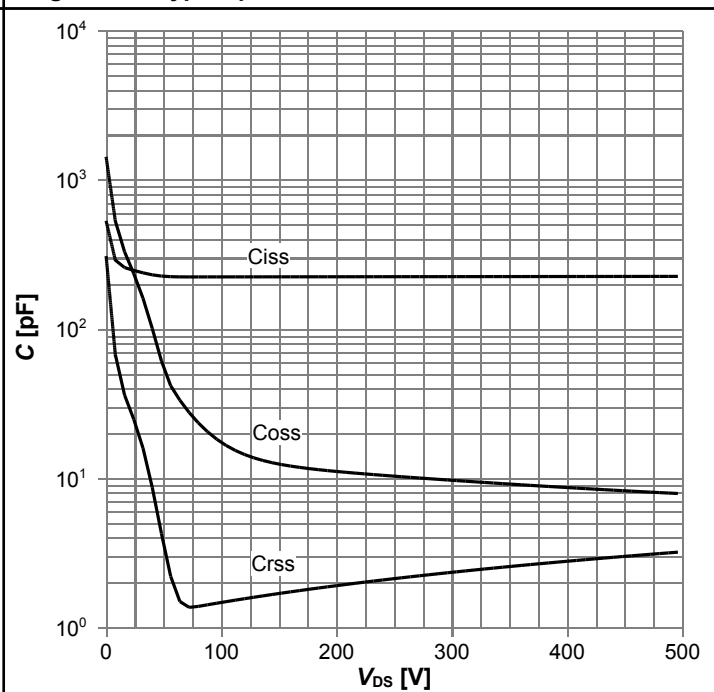
Diagram 14: Typ. capacitances
