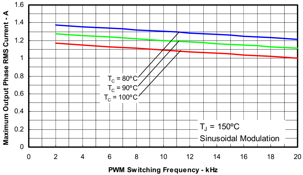
Figure 5. Maximum Sinusoidal Phase Current vs. PWM Switching Frequency Sinusoidal Modulation, V^+ = 360\text{V} , T_J = 150^\circ\text{C} , F_{\text{MOD}} = 50\text{Hz} , MI = 0.8 , PF = 0.6
