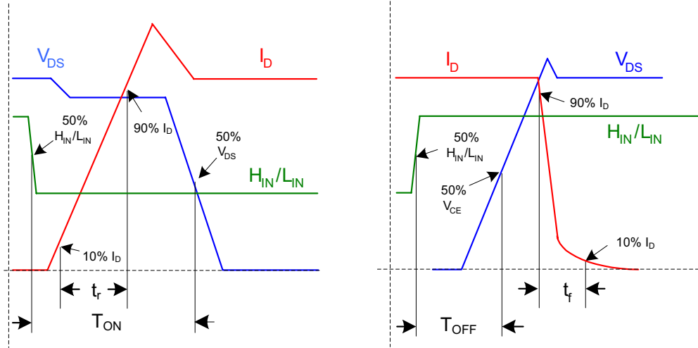
Figure 13a. Input to Output propagation turn-on delay time.
