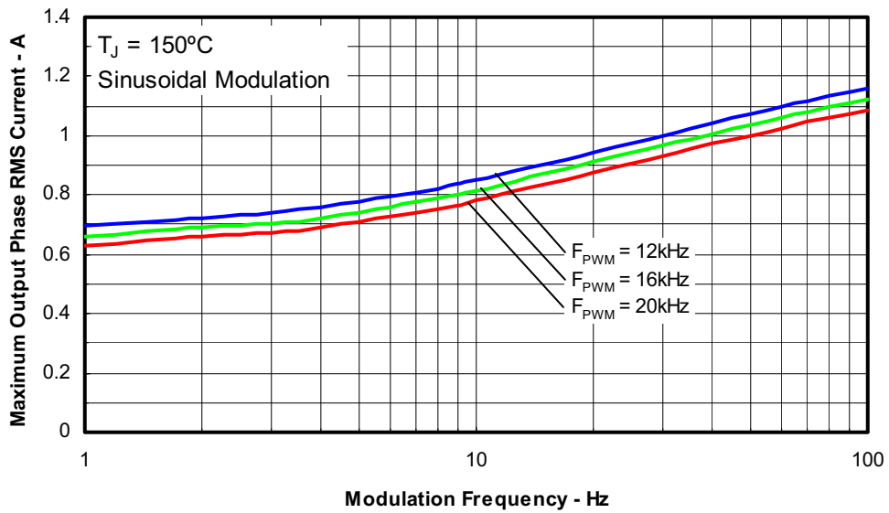
Figure 6. Maximum Sinusoidal Phase Current vs. Modulation Frequency Sinusoidal Modulation, V^+ = 360\text{V} , T_J = 150^\circ\text{C} , MI = 0.8 , PF = 0.6
