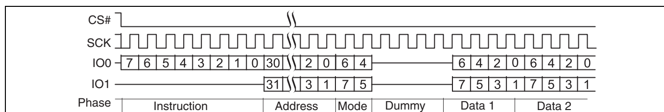
Figure 13 Dual I/O command
