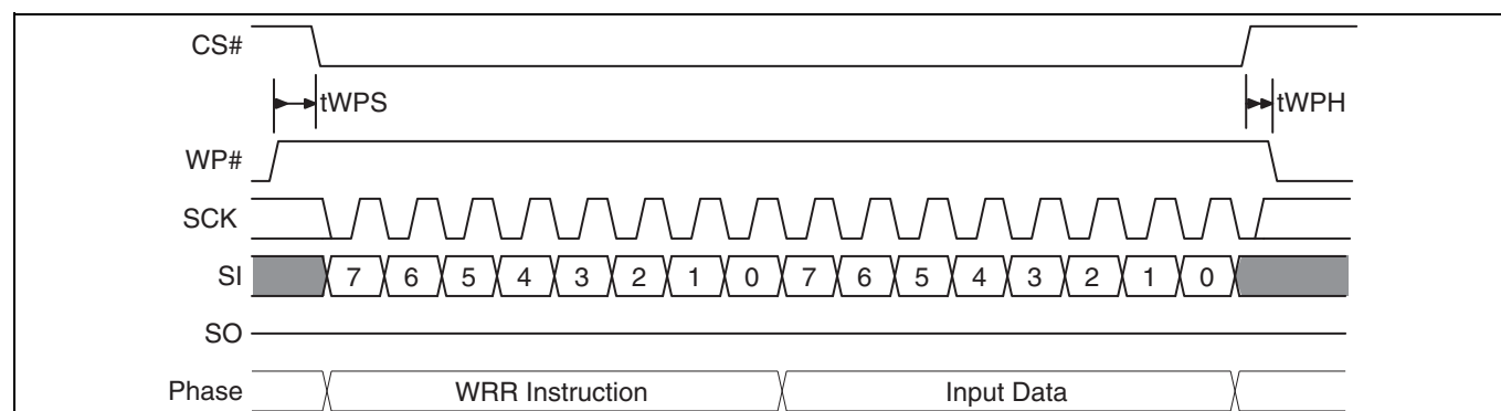
Figure 33 WP# input timing
