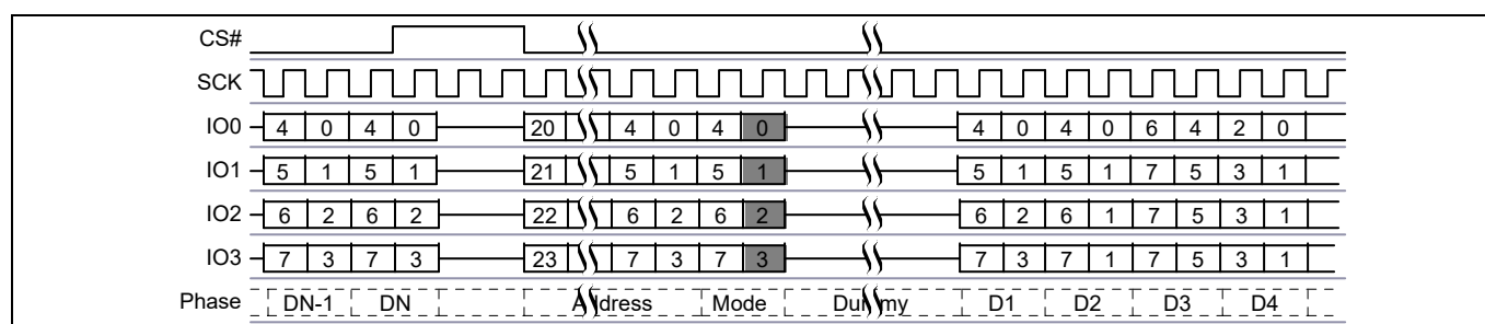
Figure 79 Continuous Quad I/O Read command sequence (3-byte address)
