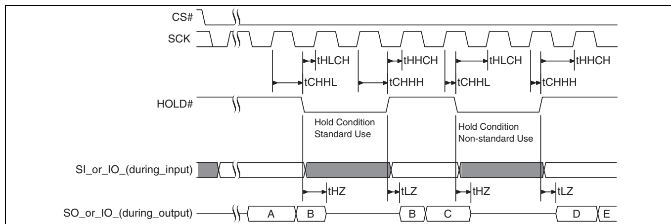
Figure 32 Hold timing
