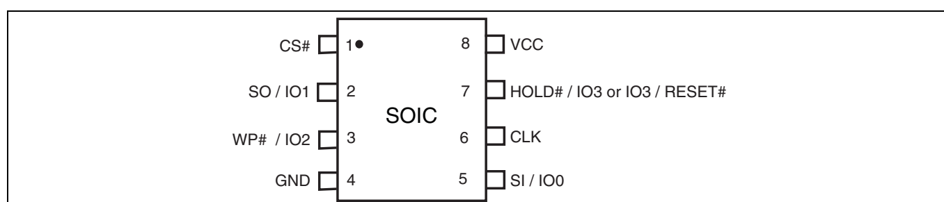
Figure 34 8-pin plastic small outline package (SO) [28]
