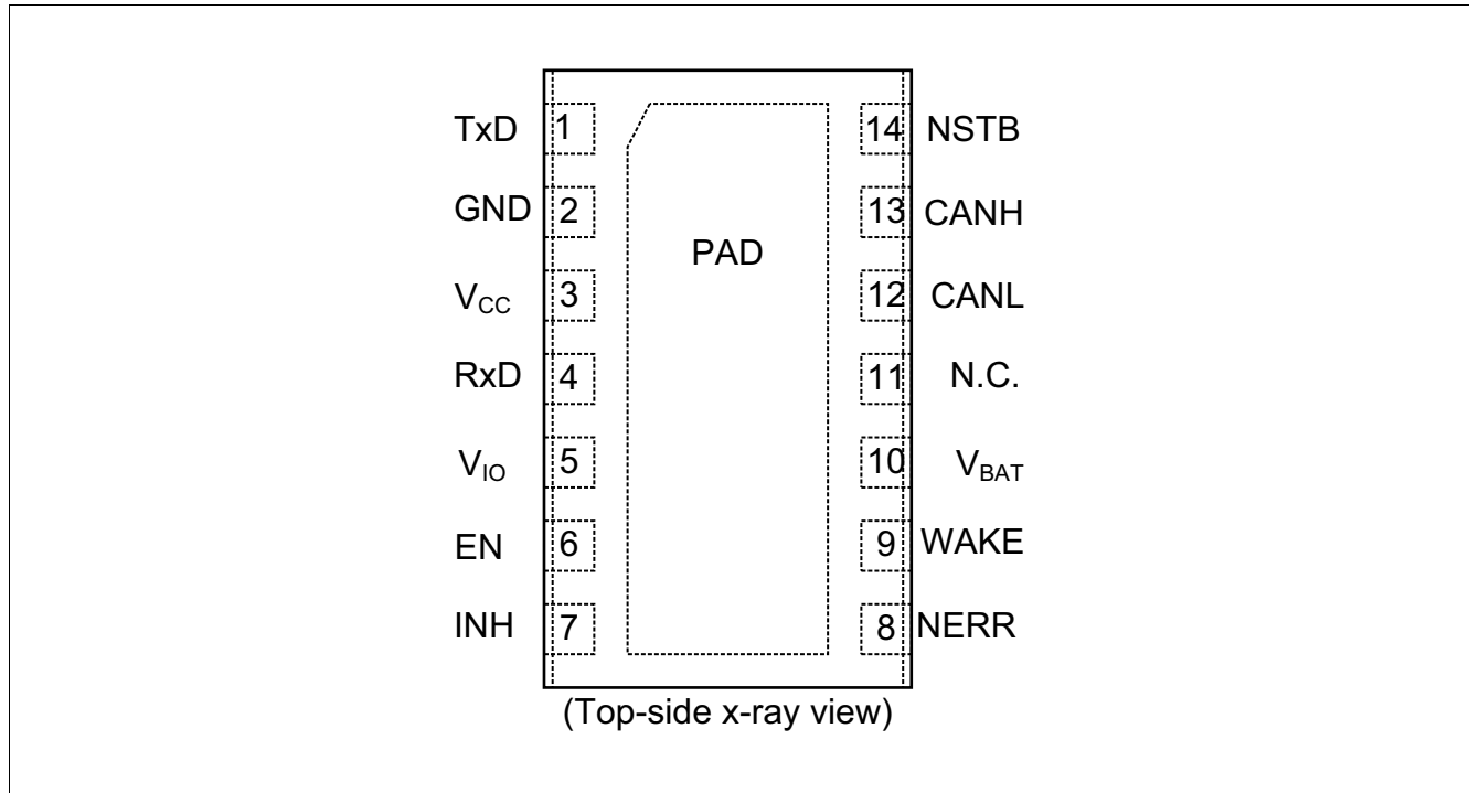
Figure 2 Pin configuration
