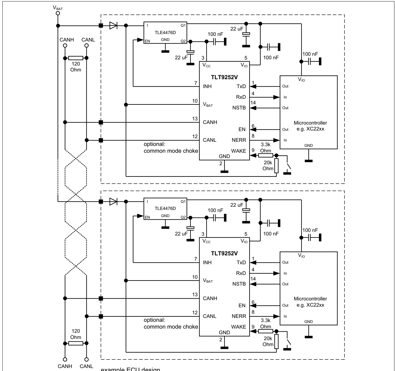
Figure 34 Application circuit
