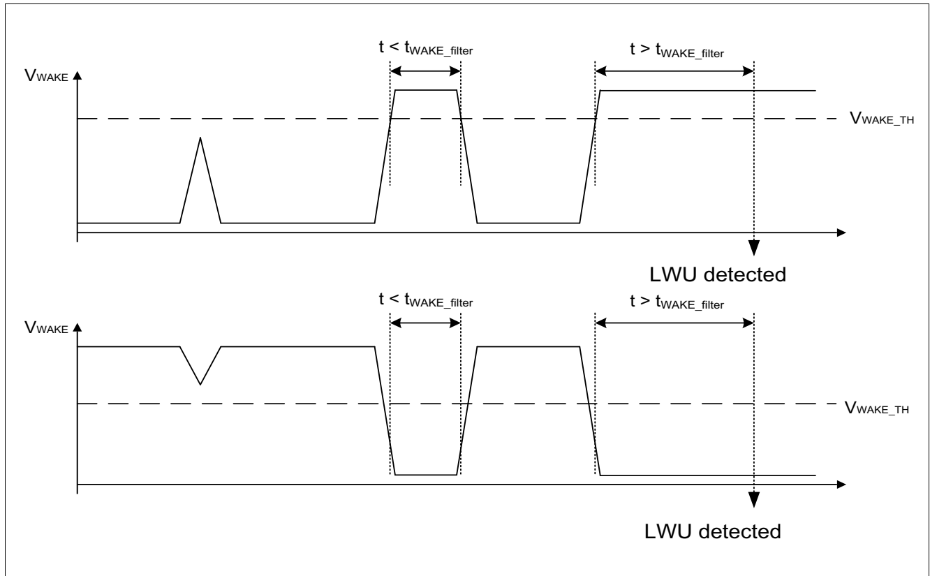
Figure 15 Local Wake-Up
