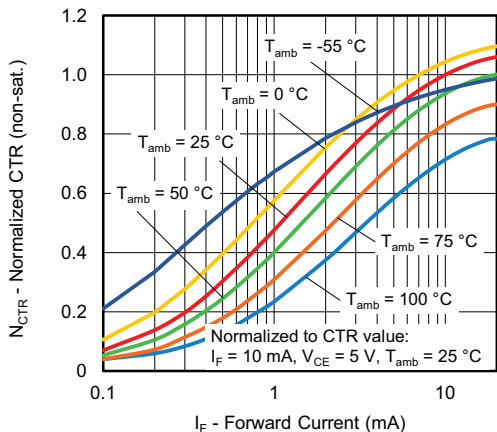
Fig. 11 - Normalized CTR (non-saturated) vs. Forward Current
