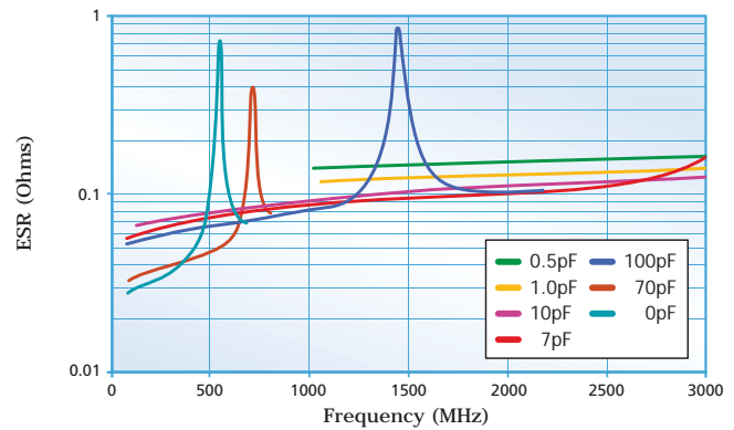
Q(MS) Series ESR vs Frequency Case size
