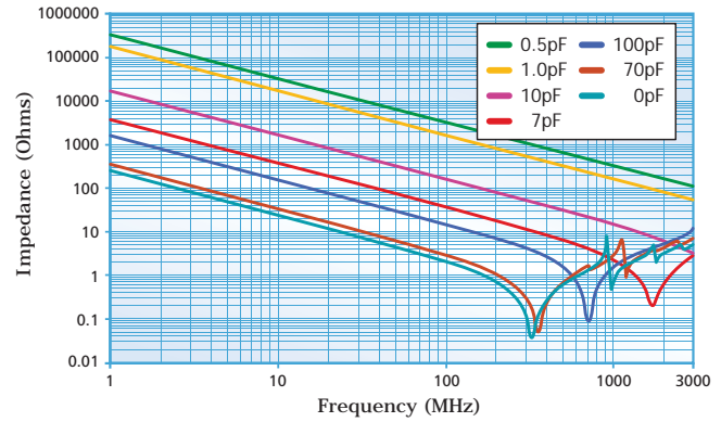
Q(MS) Series Impedance vs Frequency Case size
