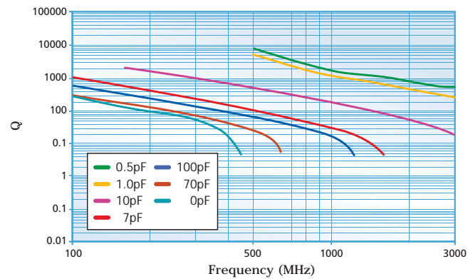
Q(MS) Series Q vs Frequency Case size
