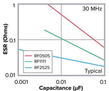
ESR vs. CAPACITANCE
