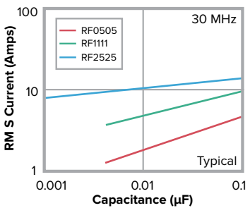
CURRENT RATING vs. CAPACITANCE
