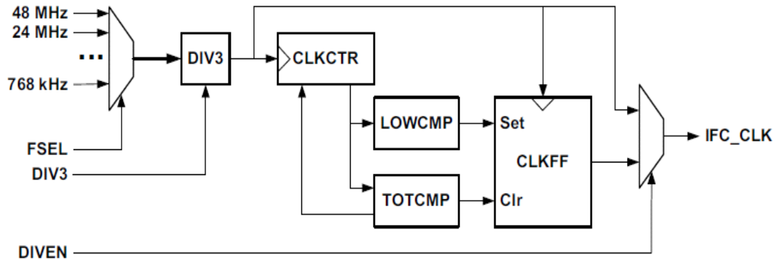
Figure 27. IO_CLK Generation
