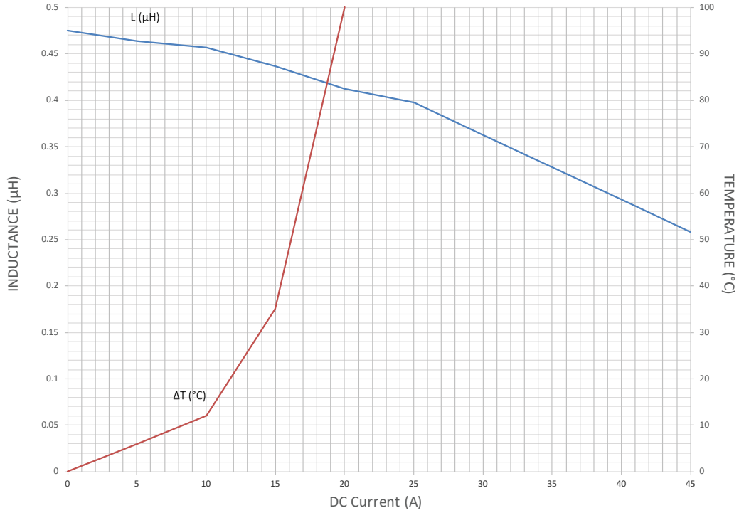
L&I Curve
