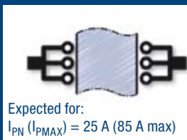
Fig. 4b. The 2 extreme possibilities for connecting the primary current circuit (as example: CAS or CASR 25-NP)
