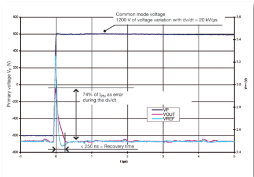
Fig. 10a. Typical common mode behaviour (1200 V of voltage variation applied with dv/dt = 20 \text{ kV}/\mu s )
