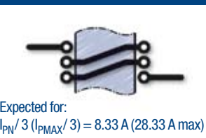
Fig. 4b. The 2 extreme possibilities for connecting the primary current circuit (as example: CAS or CASR 25-NP)
