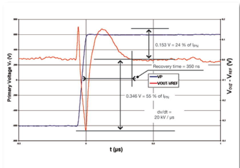
Fig. 10b. CASR 50-NP ; Typical common mode behaviour ; V_{OUT} - V_{REF} ; (1200 V of voltage variation applied with dv/dt = 20 \text{ kV}/\mu s )
