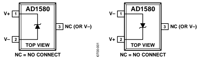
Figure 1. SOT-23
