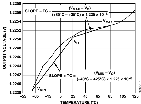
Figure 13. Output Voltage vs. Temperature
