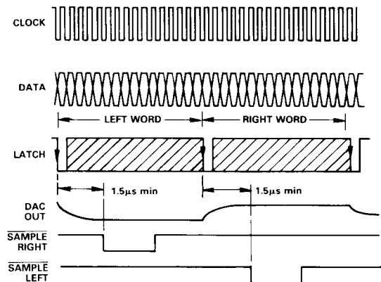
Figure 10. Control Signals for One DAC Circuit
