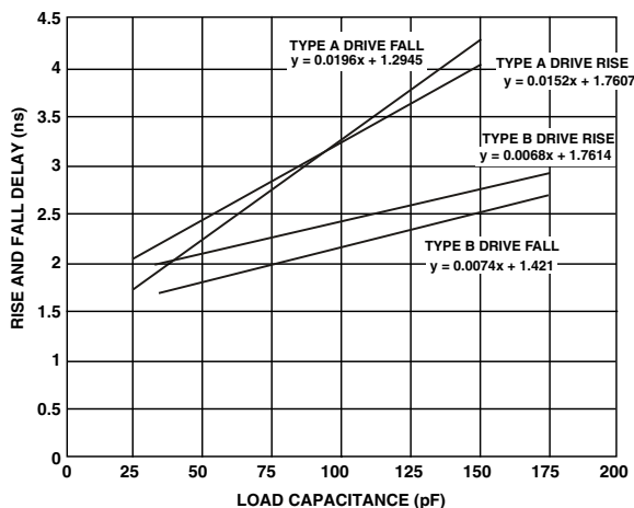
Figure 45. Typical Output Rise/Fall Delay ( V_{DD\_EXT} = \text{Max} )
