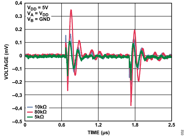
Figure 32. Digital Feedthrough
