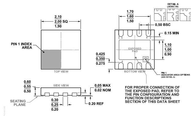
Figure 51. 8-Lead Frame Chip Scale Package [LFCSP] 2.00 mm x 2.00 mm Body and 0.55 mm Package Height (CP-8-10)
