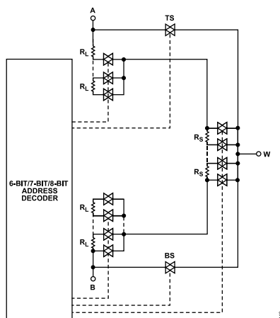
Figure 46. AD5110/AD5112/AD5114 Simplified RDAC Circuit
