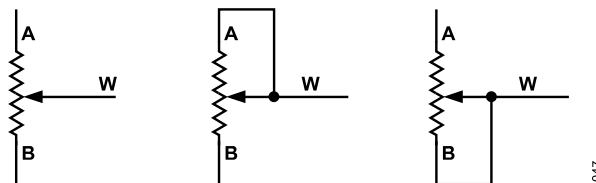
Figure 47. Rheostat Mode Configuration
