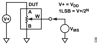
Figure 36. Potentiometer Divider Nonlinearity Error (INL, DNL)
