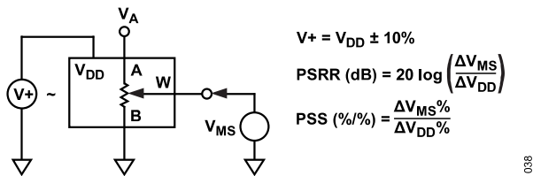
Figure 38. Power Supply Sensitivity (PSS, PSRR)
