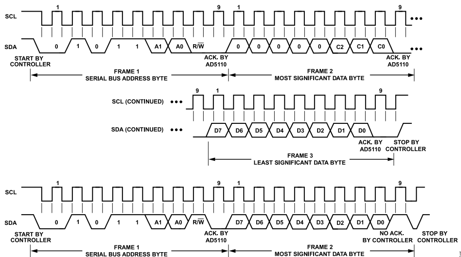
Figure 45. AD5110 Interface Read Command
