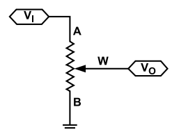
Figure 48. Potentiometer Mode Configuration
