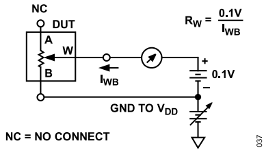
Figure 37. Wiper Resistance
