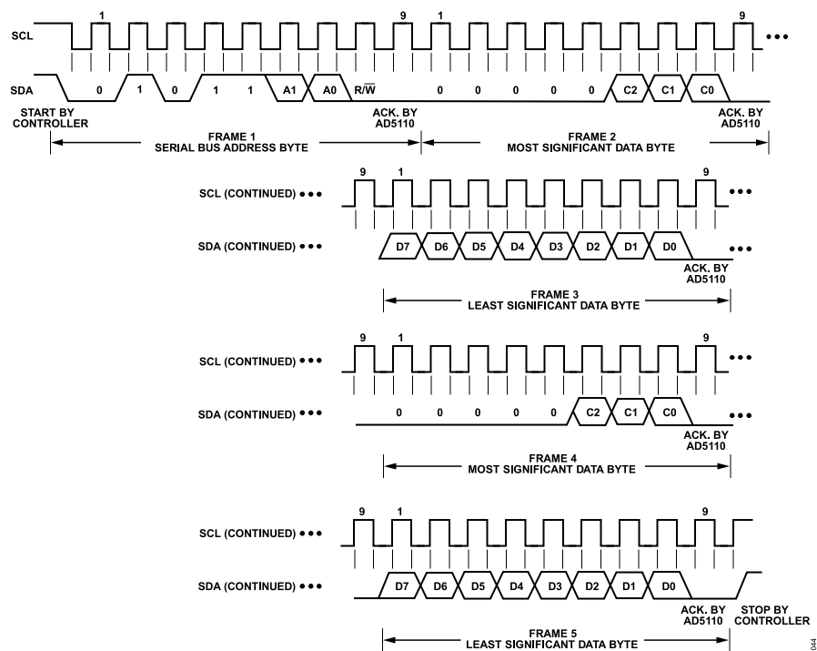
Figure 44. AD5110 Interface Multiple Write
