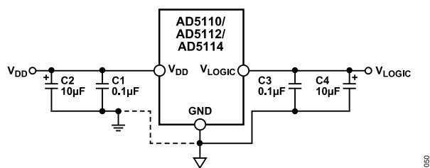
Figure 50. Power Supply Bypassing
