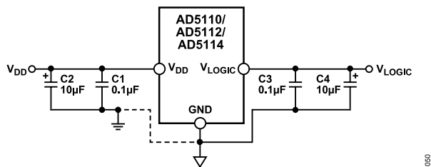
Figure 50. Power Supply Bypassing
