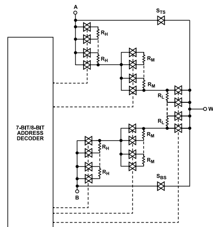
Figure 49. AD5124/AD5144/AD5144A Simplified RDAC Circuit
