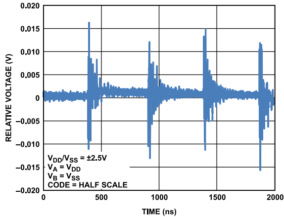
Figure 36. Digital Feedthrough
