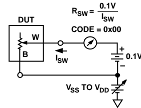
Figure 35. Test Circuit for Incremental On Resistance
