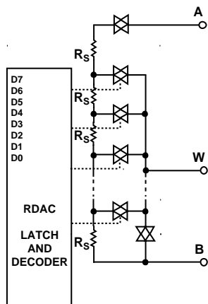
Figure 39. Equivalent RDAC Circuit
