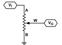
Figure 41. Potentiometer Mode Configuration
