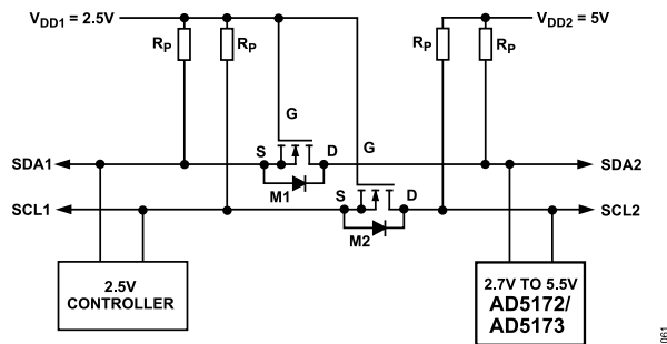
Figure 52. Level Shifting for Different Voltage Operation
