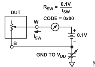
Figure 35. Incremental On Resistance
