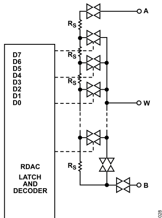
Figure 40. AD5172/AD5173 Equivalent RDAC Circuit
