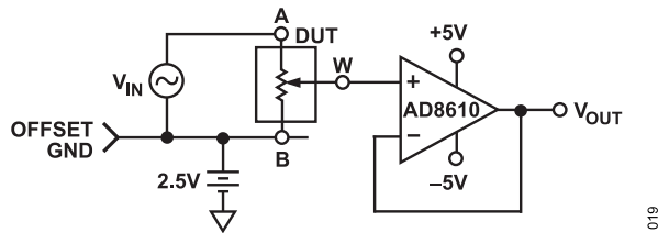
Figure 34. Test Circuit for Gain vs. Frequency
