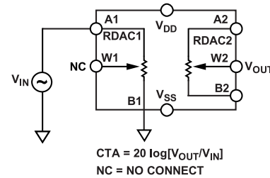
Figure 37. Analog Crosstalk
