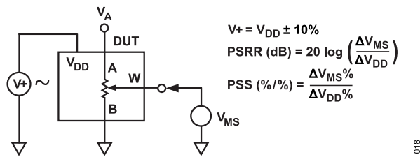
Figure 33. Power Supply Sensitivity (PSS, PSSR)
