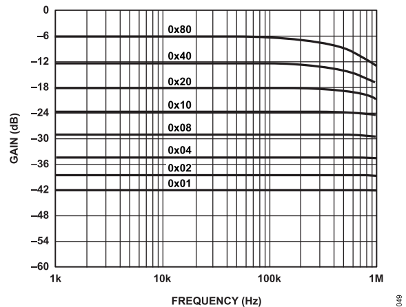
Figure 20. Gain vs. Frequency vs. Code, R_{AB} = 10\text{ k}\Omega
