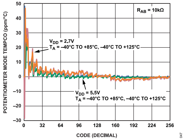
Figure 18. AD5172 Potentiometer Mode Tempco \Delta V_{WB}/\Delta T vs. Code
