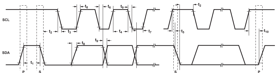
Figure 3. I 2 C Interface Detailed Timing Diagram
