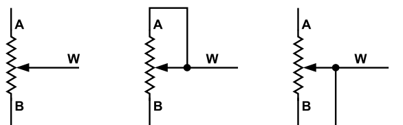
Figure 39. Rheostat Mode Configuration
