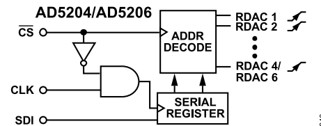
Figure 33. Equivalent Input Control Logic
