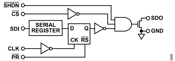
Figure 34. Detail SDO Output Schematic of the AD5204
