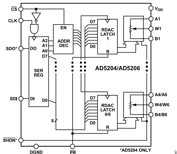
Figure 32. Block Diagram
