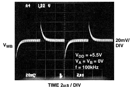
Figure 18. Digital Feedthrough
