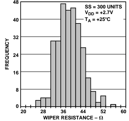
Figure 6. Wiper Contact Resistance
