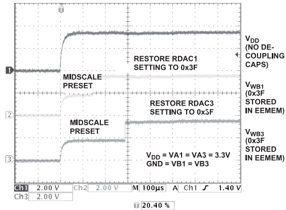
Figure 20. t_{EMEM\_RESTORE} of RDAC1 and RDAC3
