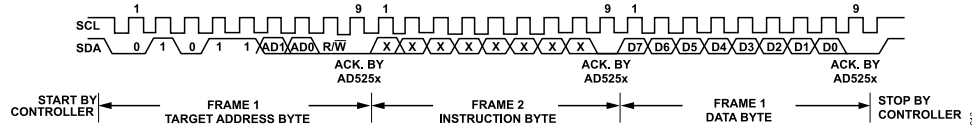
Figure 33. General I 2 C Write Pattern
