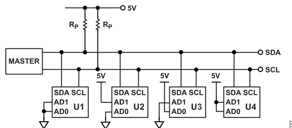
Figure 37. Multiple AD5251/AD5252 Devices on a Single Bus
