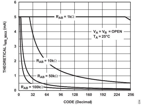
Figure 22. AD5252 I_{WB\_MAX} vs. Code
