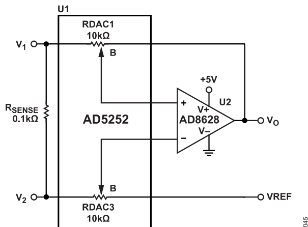
Figure 45. Current-Sensing Amplifier
