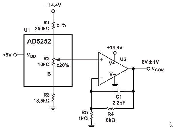
Figure 44. Apply 5 V Digital Potentiometer AD5251 in a 6 V \pm 1 V Application
