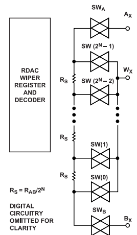
Figure 41. Equivalent RDAC Structure
