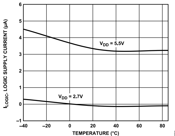
Figure 17. Logic Supply Current vs. Temperature vs. VDD
