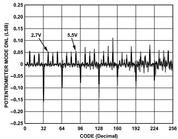
Figure 11. DNL vs. Code vs. Supply Voltage
