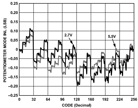
Figure 10. INL vs. Supply Voltages
