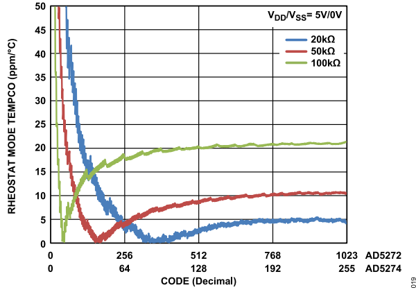
Figure 24. Tempco \Delta R_{W/A}/\Delta T vs. Code
