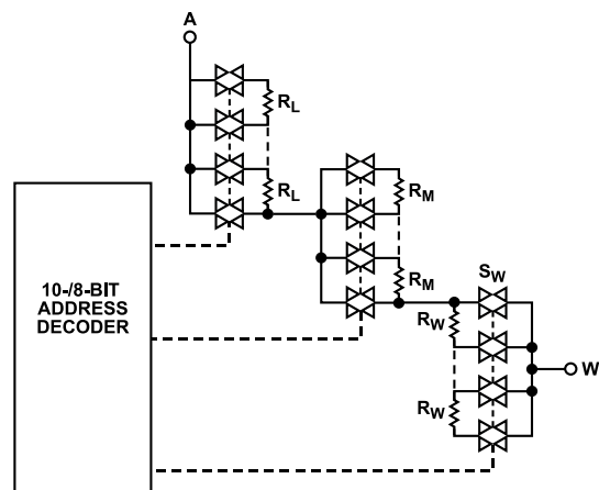
Figure 46. Simplified RDAC Circuit
