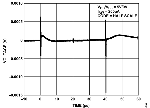
Figure 35. Digital Feedthrough
