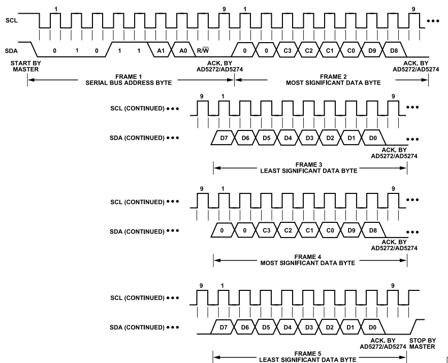
Figure 44. Multiple Write
