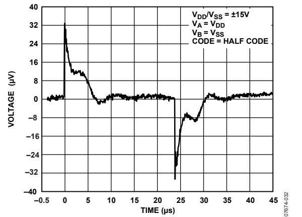
Figure 53. Digital Feedthrough
