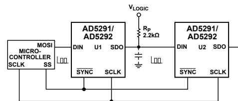
Figure 64. Daisy-Chain Configuration Using SDO
