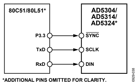
Figure 38. AD5304/AD5314/AD5324 to 80C51/80L51 Interface
