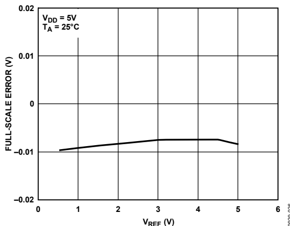
Figure 26. Full-Scale Error vs. V_{REF}
